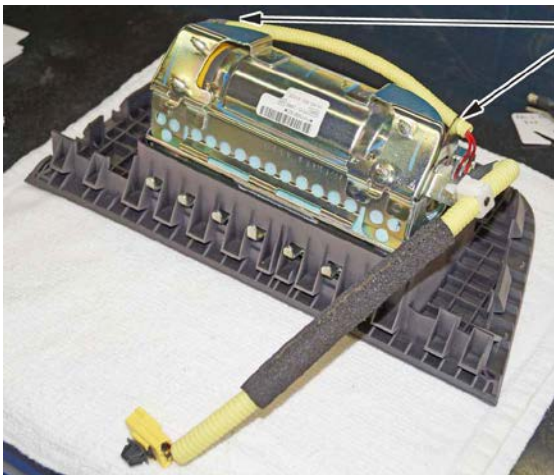
INFLATOR BRACKETS
