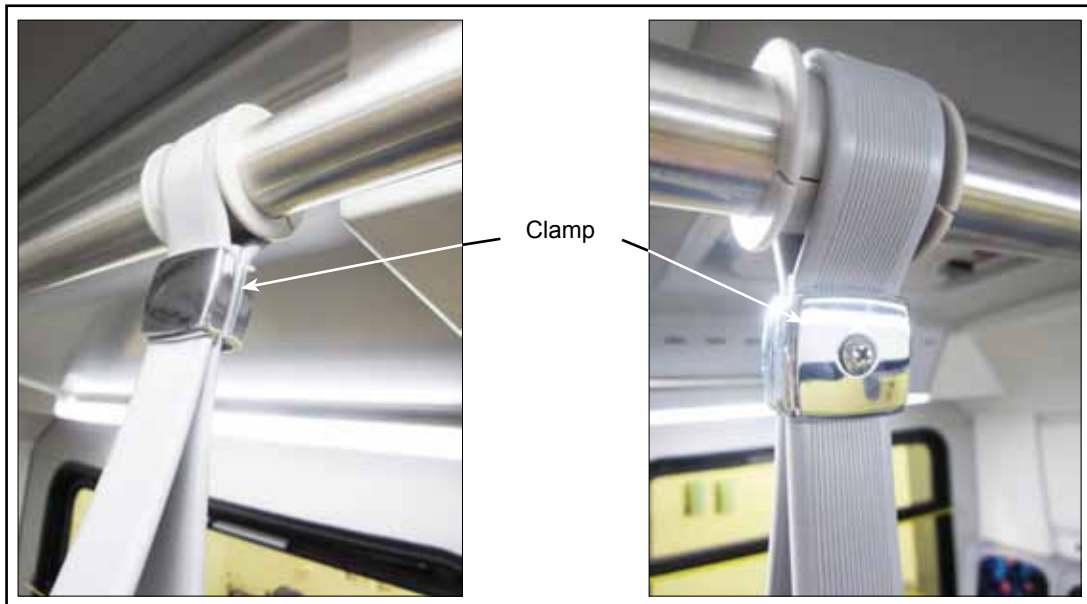
Figure 2 - Grab Handle With a Metal Clamp (Suggested Model N70020)
