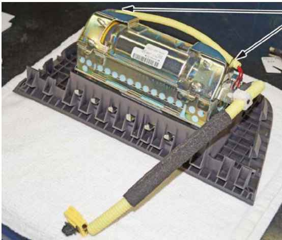
INFLATOR BRACKETS
