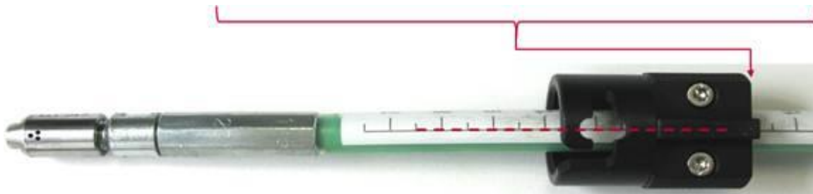
Figure 15: Arrow indicating how the back side of the adaptor must align with the scale. Red dotted line indicating how the longitudinal slot must align with the black line on the scale.
