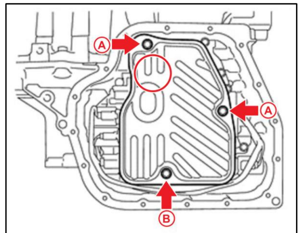
Figure 16. Oil Strainer
