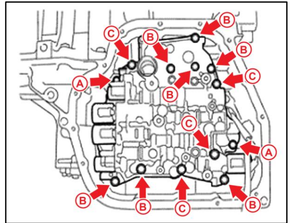
Figure 14. Transmission Valve Body
