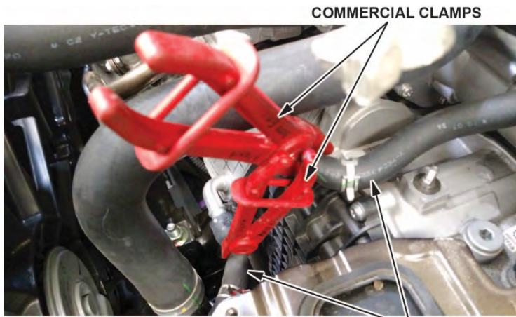
COOLANT HOSES
