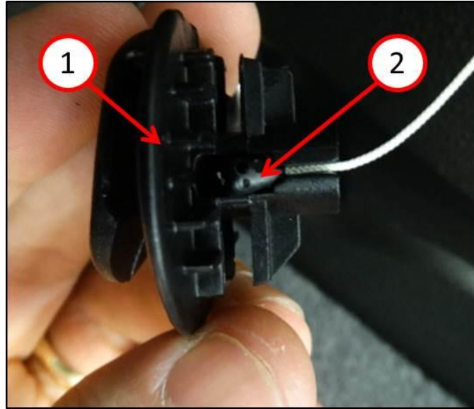
Fig. 3 Cable Insertion
