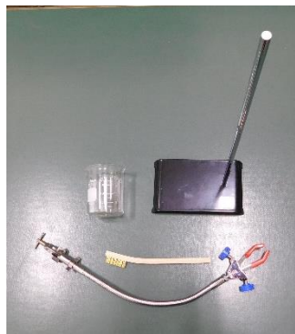
Figure 2 – Essential Tool – Injector Cleaner Accessory Kit - stand with base, arm with clamp, brass brush, and Pyrex beaker (EN-52575-50)
