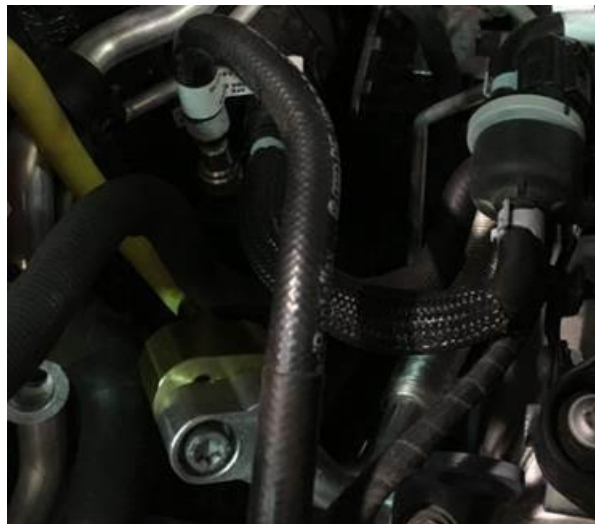
Figure 15. Attaching service station and flush hoses to rear A/C lines.
