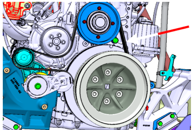
FIGURE 40: WATER PUMP DRIVEBELT
