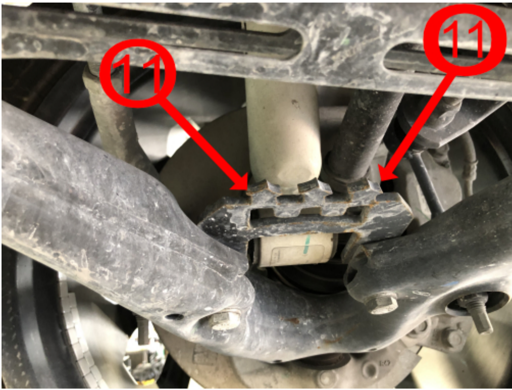
11. Aftermarket Lift Kit Block installed
