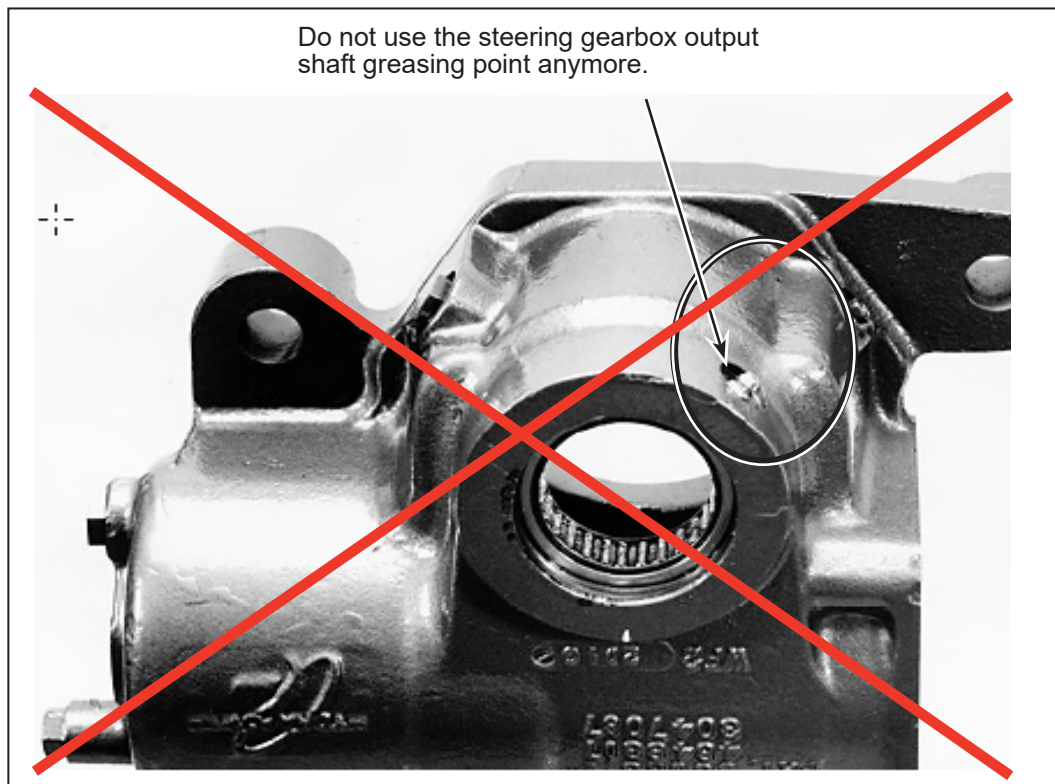
Figure 1 - Power Steering Output Shaft Greasing Zerk
