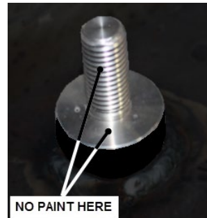
FIGURE 61: GROUND STUD #380360
