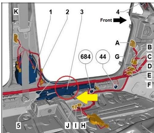
N297/N298 Connector Location. Driver side shown, passenger side similar.
