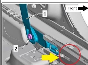
N297/N298 Connector Location. Driver side shown, passenger side similar.
