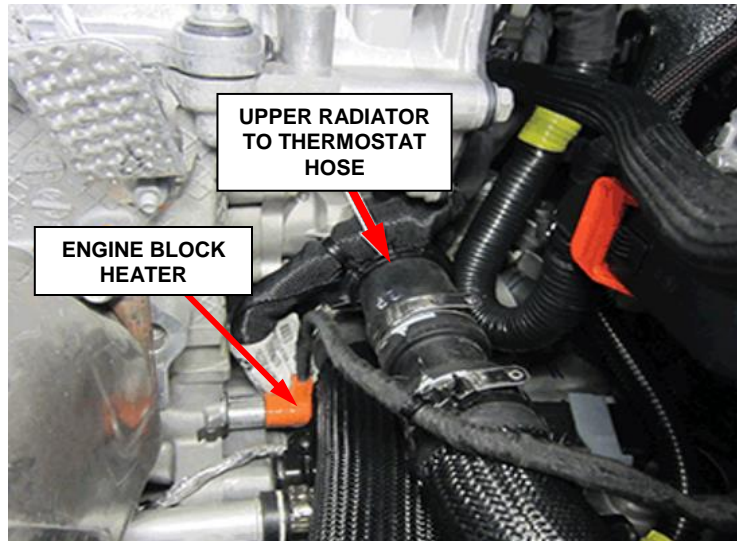
Figure 16 – Thermostat Housing
