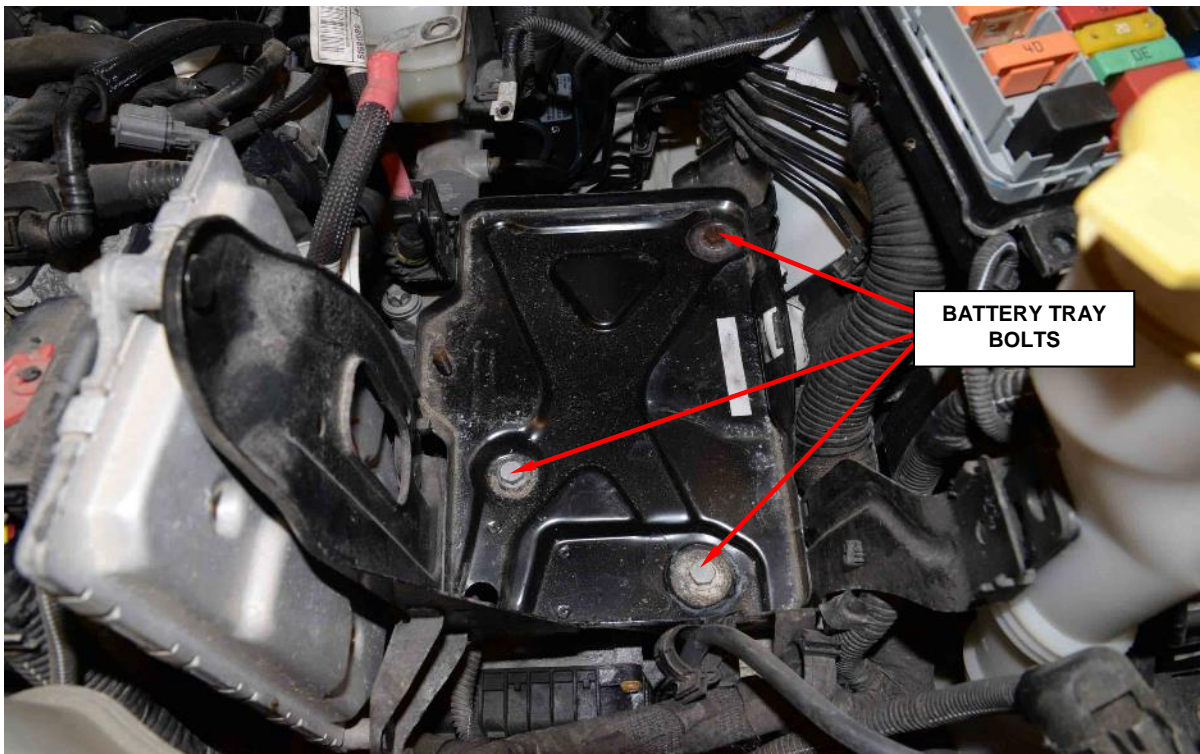
Figure 5 – Battery Tray
