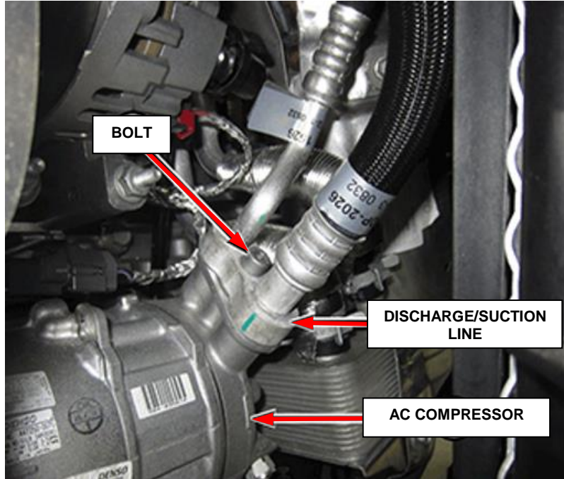
Figure 12 – AC Lines
