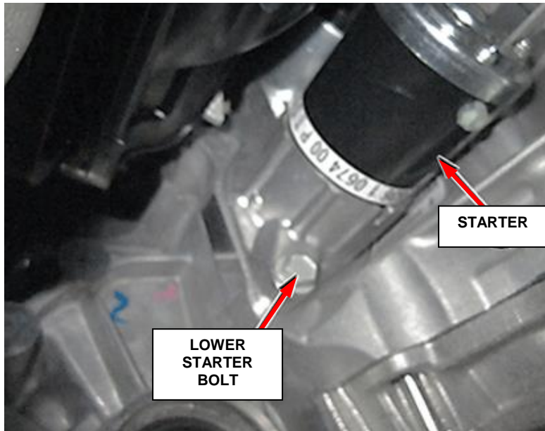
Figure 48 - Starter
