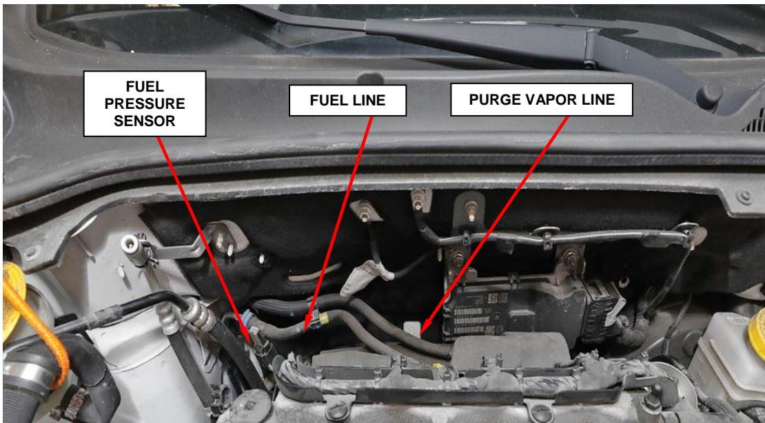
Figure 14 – Fuel Line
