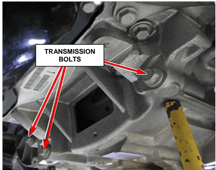
Figure 46 – Transmission Bolts
