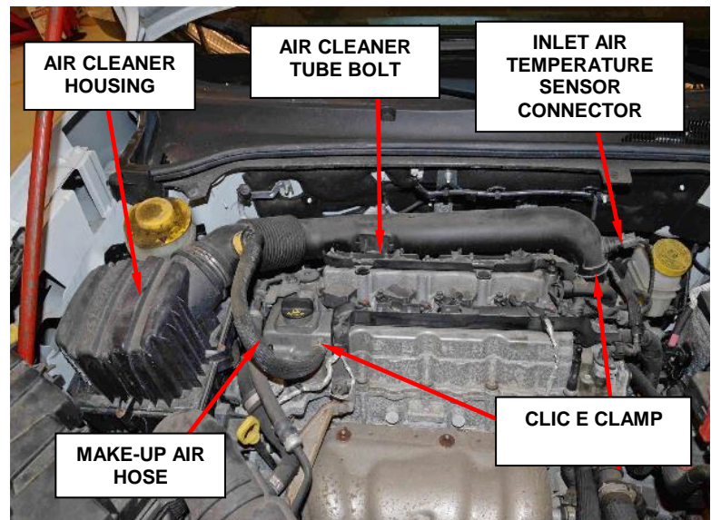
Figure 4 – Air Intake
