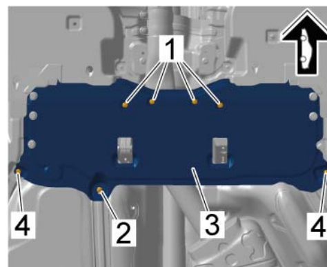
Rear centre underbody cover
