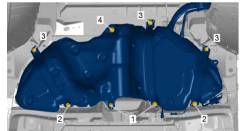
Tightening sequence for tank fastening strap
