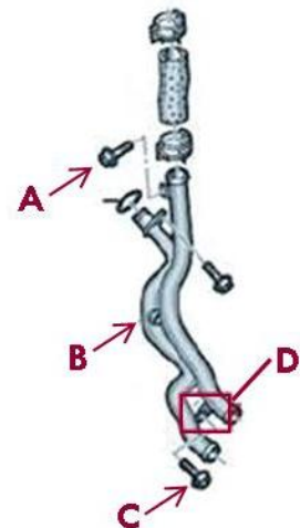
Figure 7. Loosening the coolant tube
