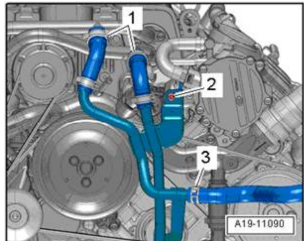
Figure 5. Front coolant pipes to be removed for 3.0T
