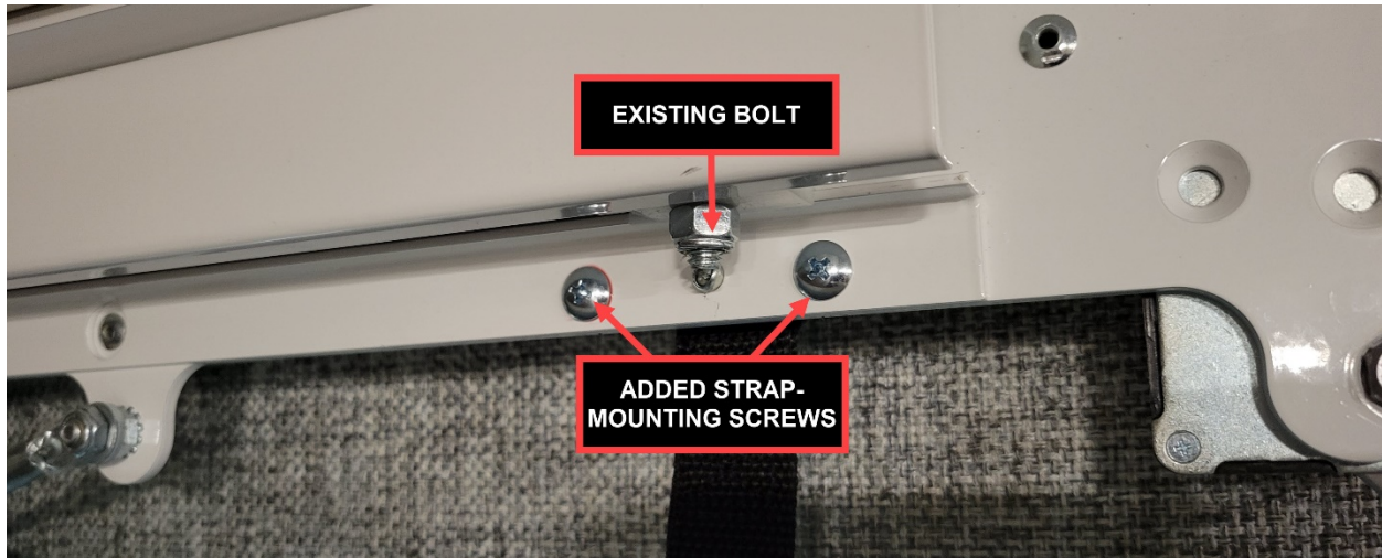
Inside of Upper Frame with Bunk Open
