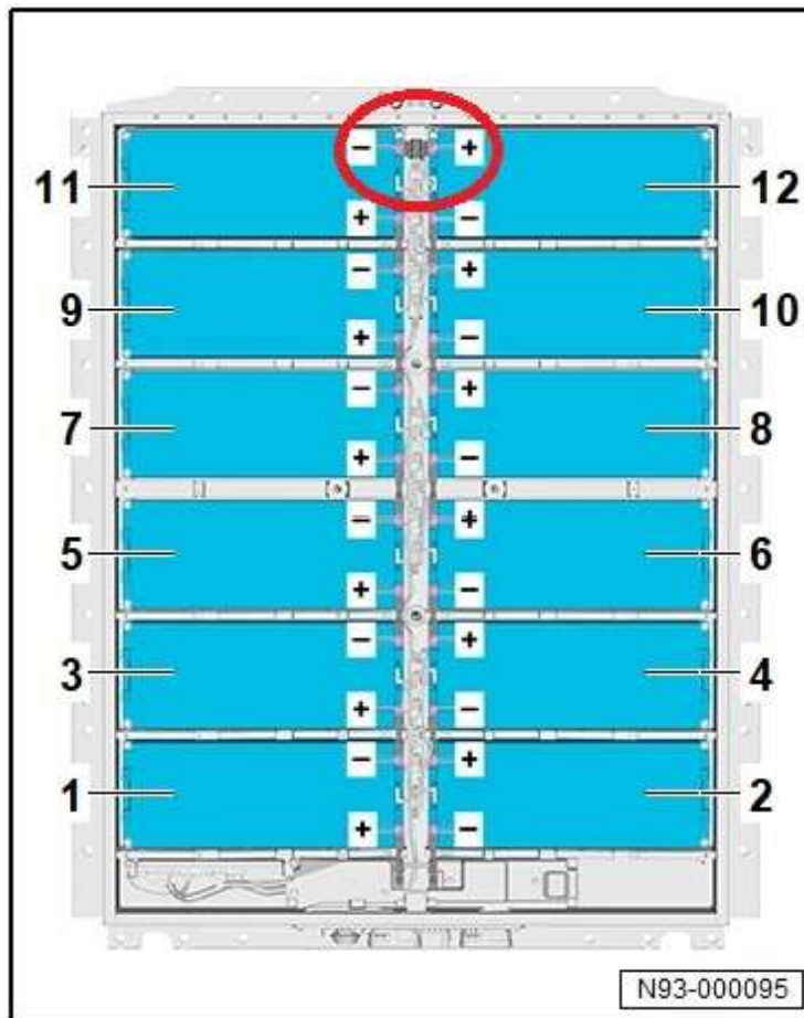
Figure 2. High-voltage connector is positioned opposite the coolant connection.
