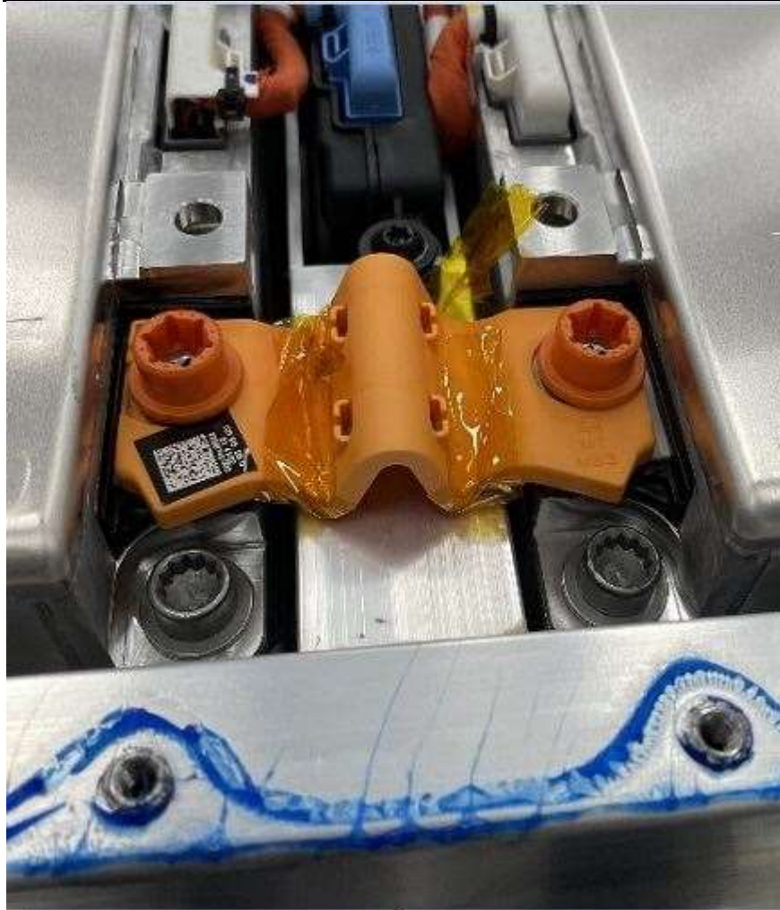
Figure 1. High-voltage connector wrapped in adhesive tape
