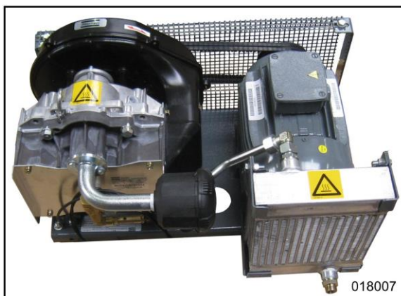
Figure 1: "Atlas Copco SFR4" air compressor
