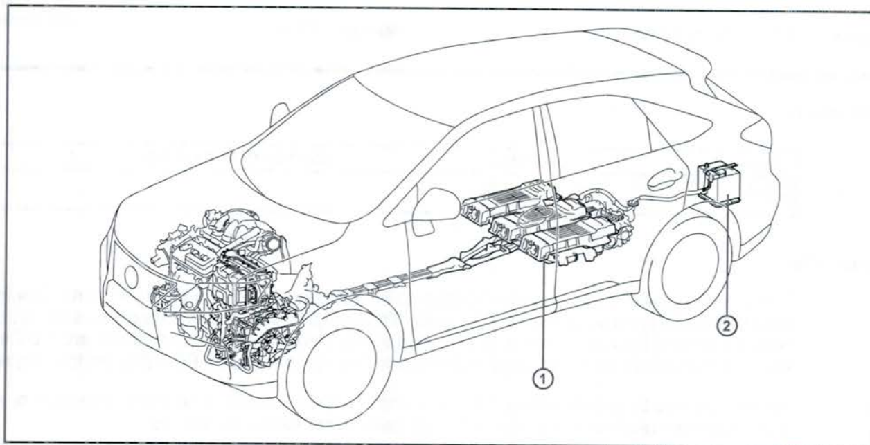
Figure 1. High-Voltage Components and Cables
