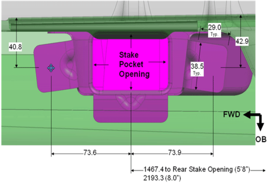
Figure 3 – Top View - Front Structure
