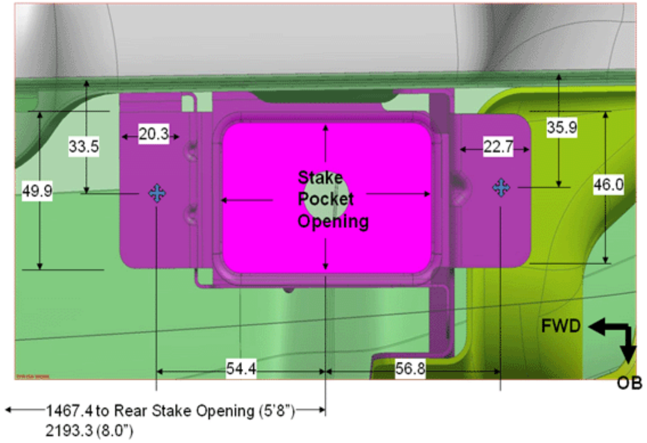
Figure 4 – Top View - Rear Structure
