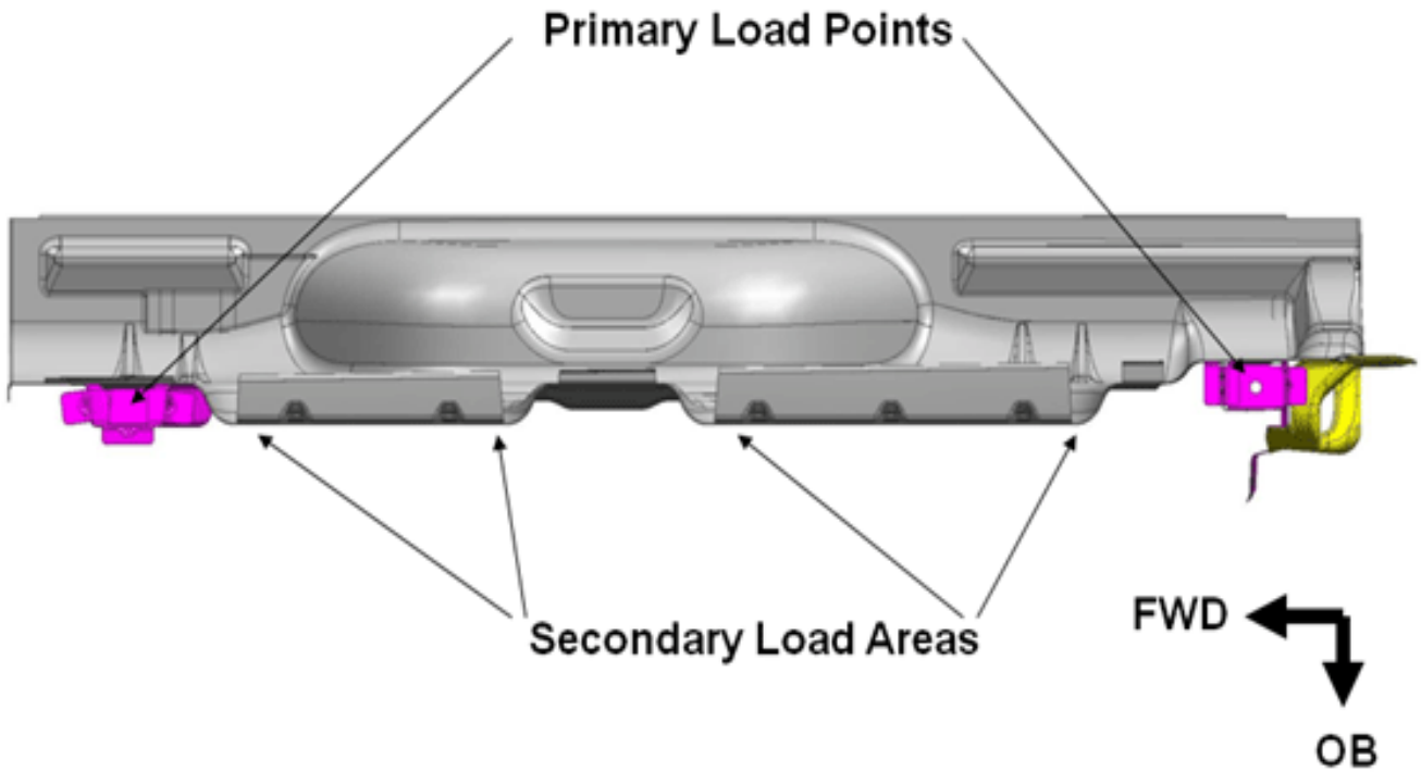
Figure 2 – Top View - Structural Members
