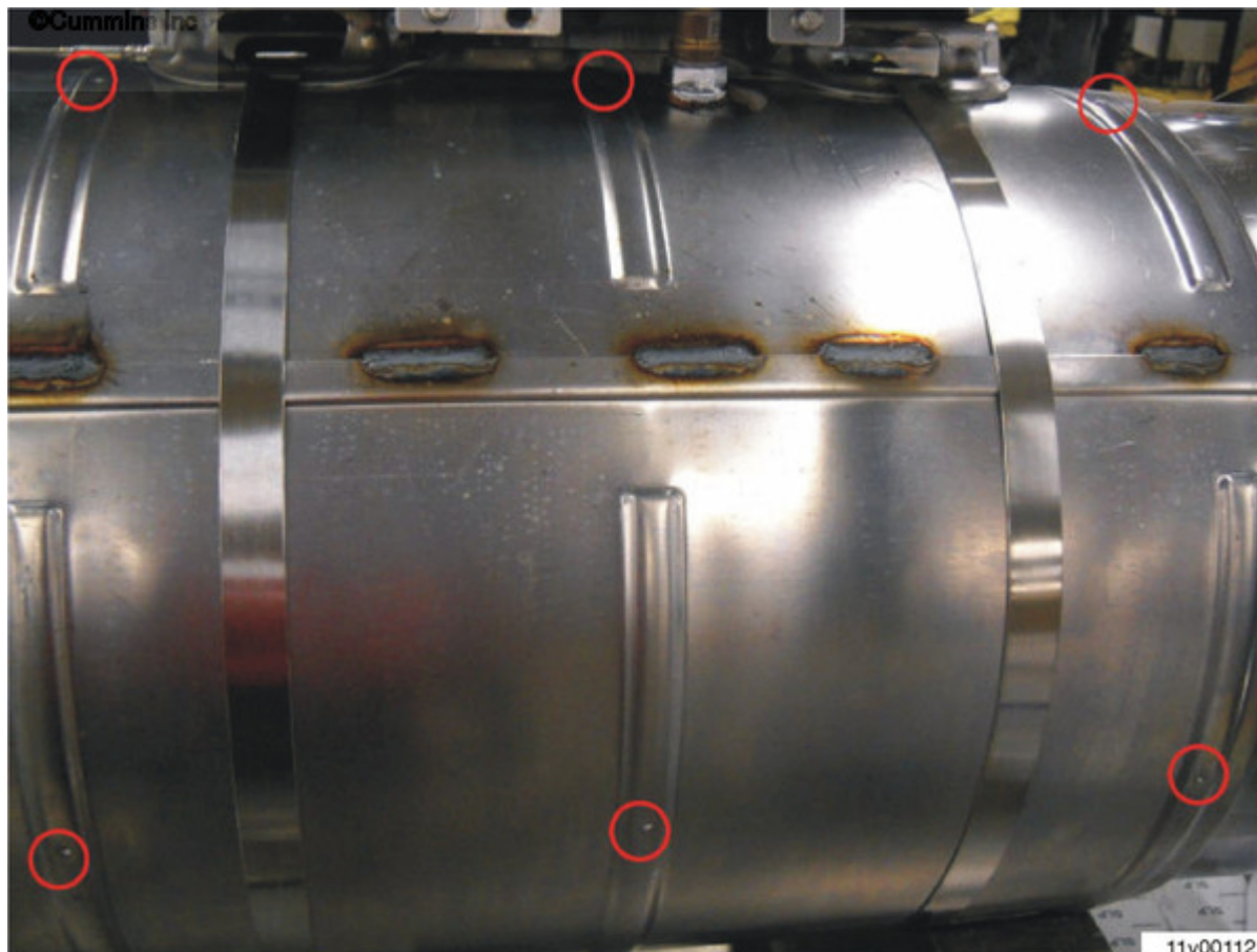
Figure 1, There are identifying dimples in the heat shield of the compatible SCR catalyst. These dimples go all the way around the SCR catalyst. They can be found in 3 different places around the circumference.
