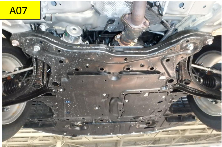
Cross member (view from rear to front) Overview
