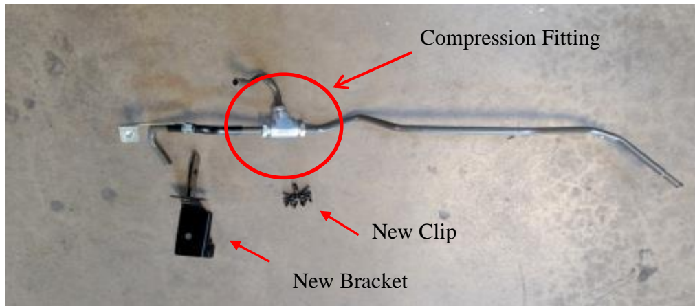
Figure 2 – New Style DEF Coolant Pipe Assembly, Frame Bracket and Clip.
